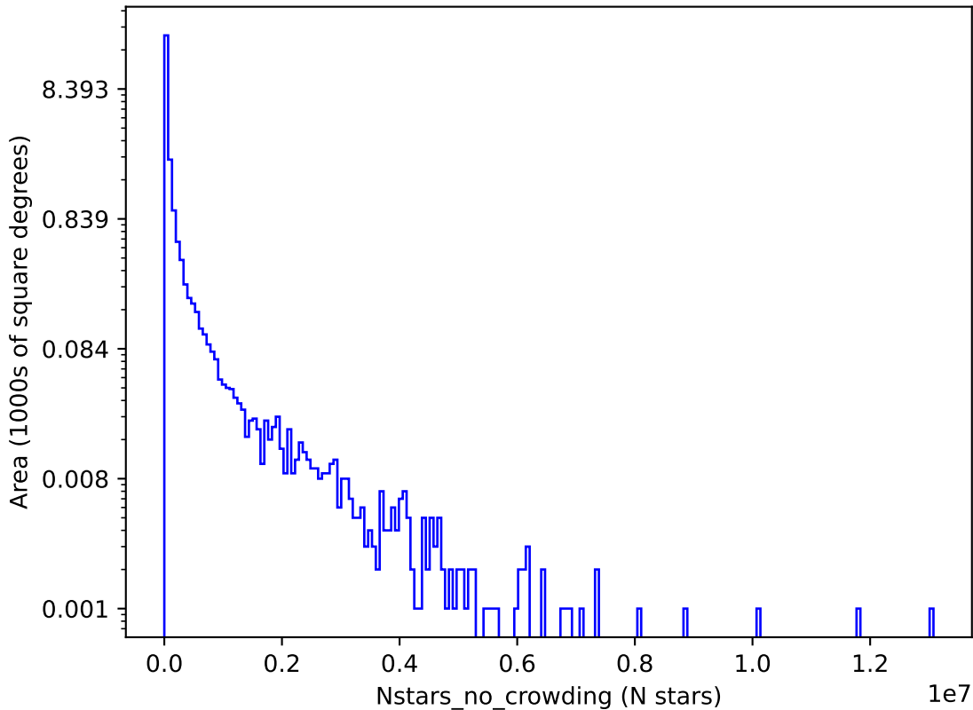
baseline_v3.2_10yrs g: Nstars_no_crowding
