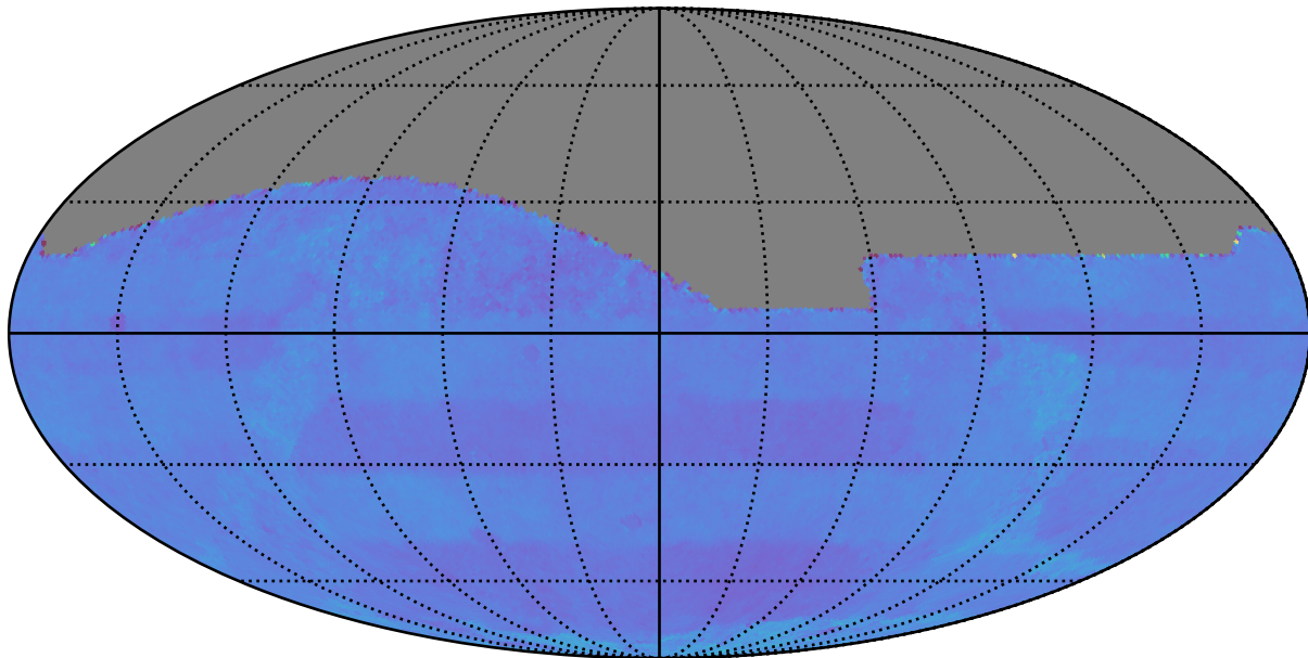
baseline_v3.2_10yrs : Normalized Proper Motion Uncert @ 24.0
