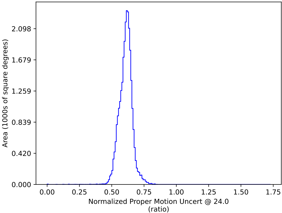
baseline_v3.2_10yrs : Normalized Proper Motion Uncert @ 24.0
