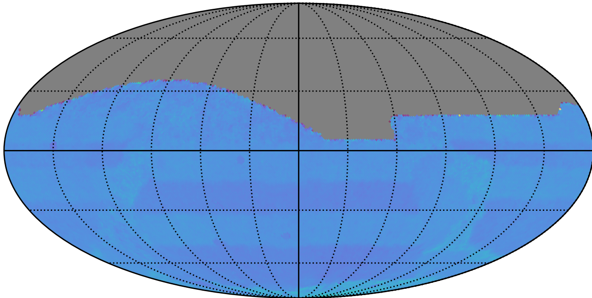
baseline_v3.2_10yrs : Normalized Proper Motion Uncert @ 20.5
