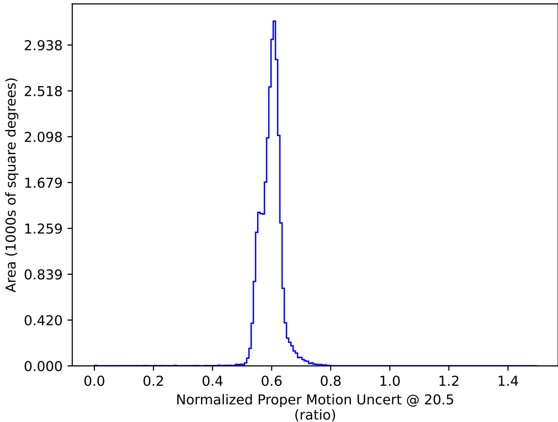
baseline_v3.2_10yrs : Normalized Proper Motion Uncert @ 20.5
