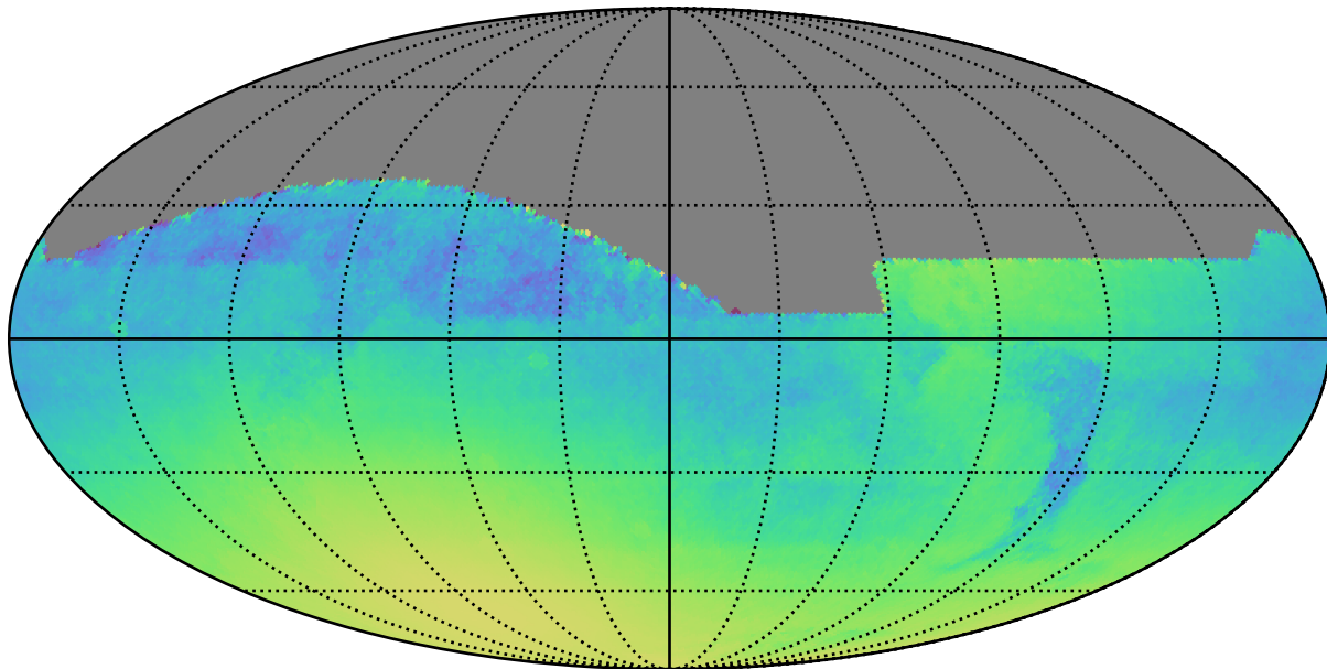
baseline_v3.2_10yrs : Normalized Parallax Uncert @ 24.0
