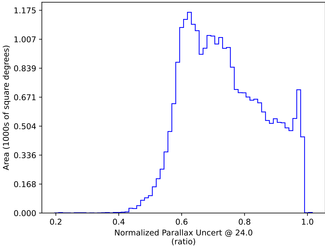
baseline_v3.2_10yrs : Normalized Parallax Uncert @ 24.0
