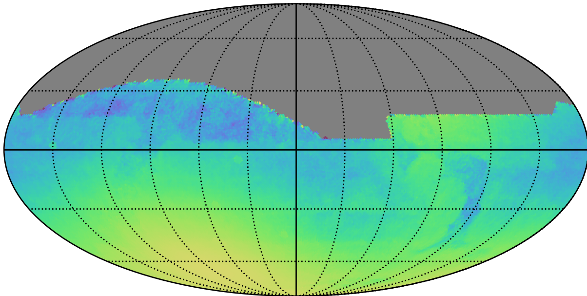
baseline_v3.2_10yrs : Normalized Parallax Uncert @ 22.4
