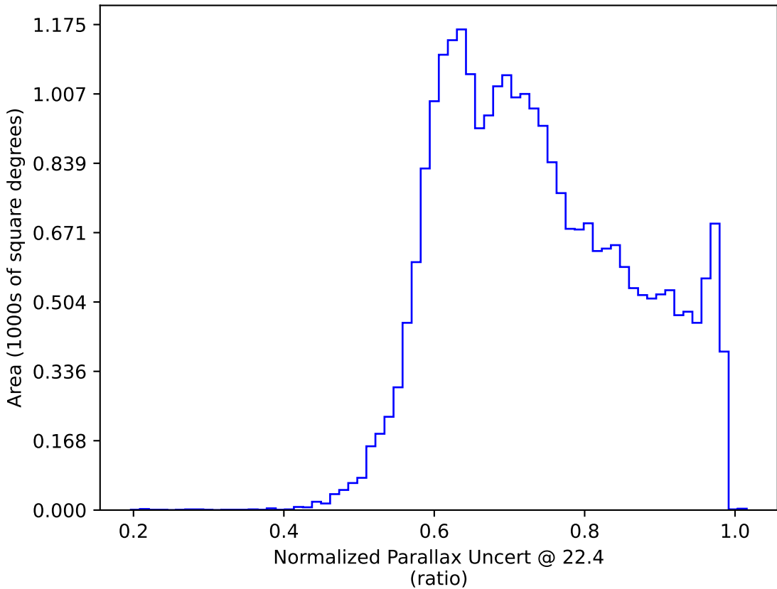
baseline_v3.2_10yrs : Normalized Parallax Uncert @ 22.4
