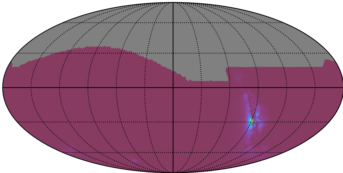
baseline_v3.2_10yrs : NlcPoints
