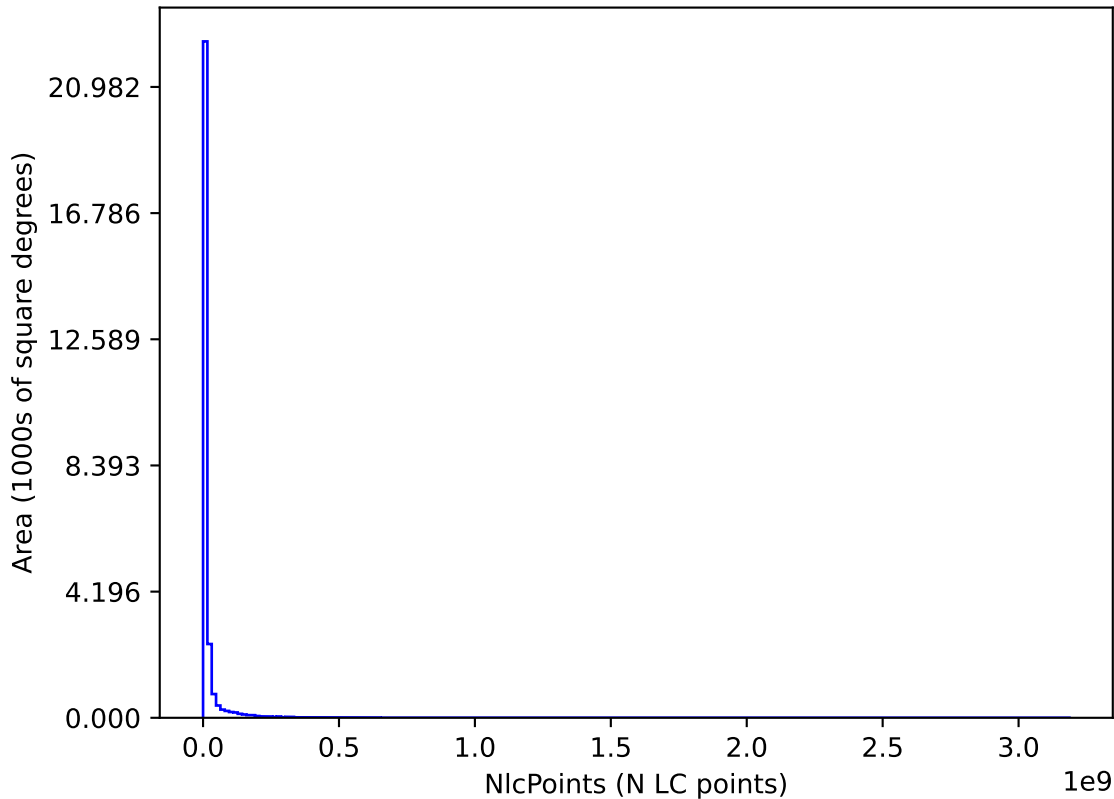
baseline_v3.2_10yrs : NlcPoints
