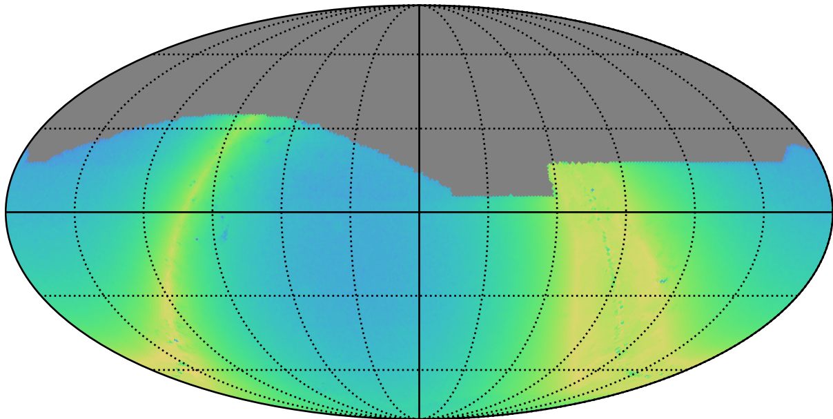
baseline_v3.2_10yrs z: N stars to Precision 0.20
