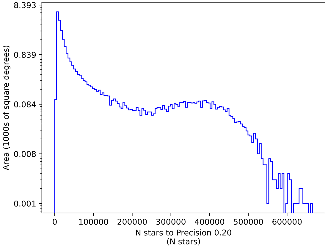
baseline_v3.2_10yrs z: N stars to Precision 0.20
