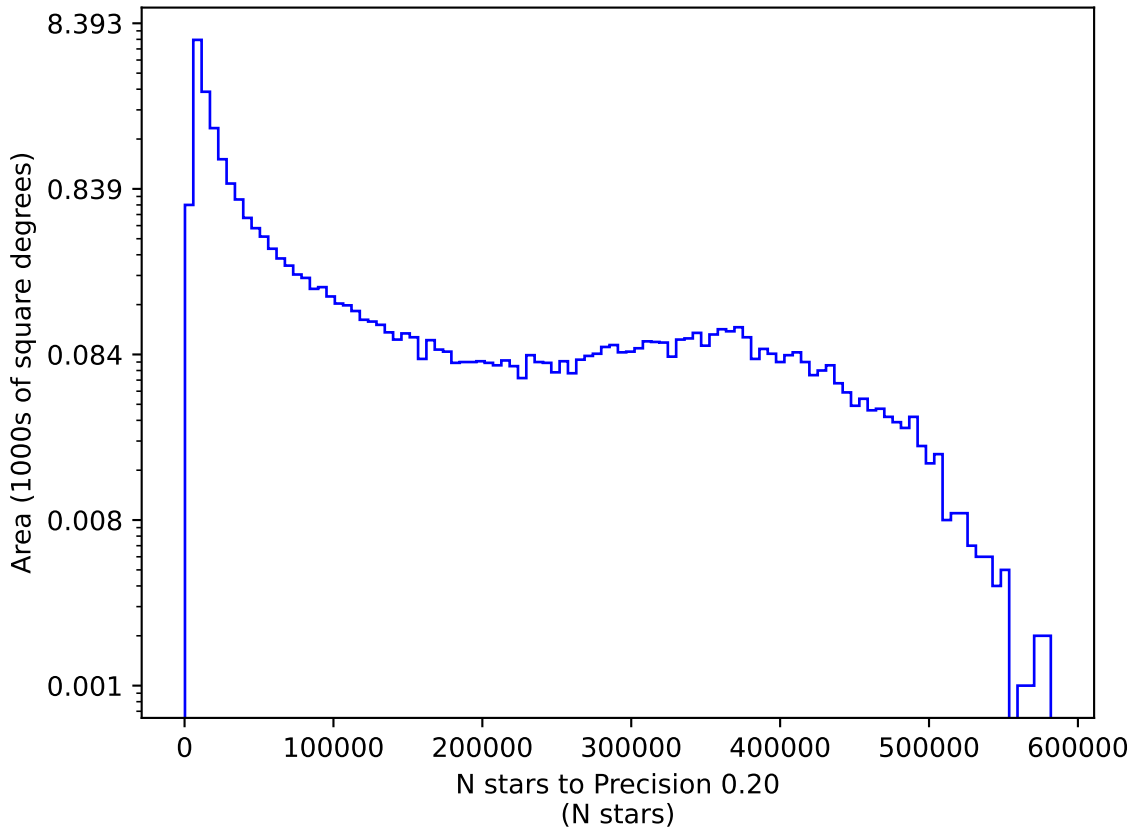
baseline_v3.2_10yrs y: N stars to Precision 0.20
