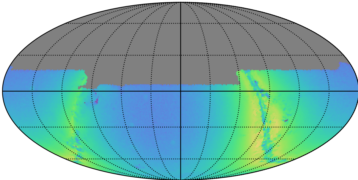
baseline_v3.2_10yrs u: N stars to Precision 0.20
