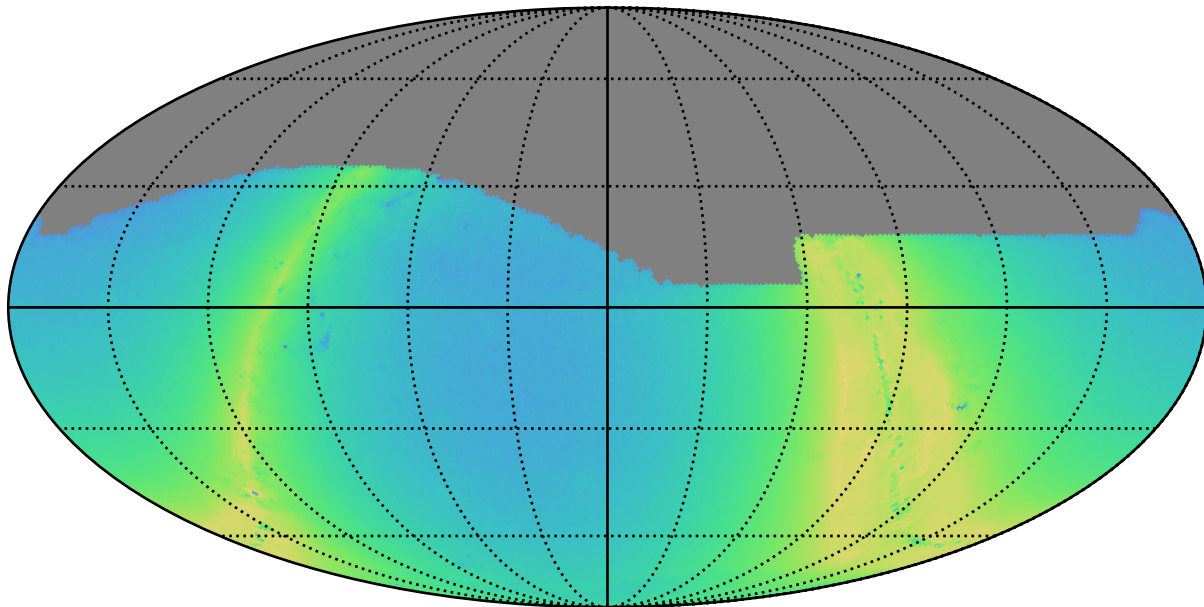
baseline_v3.2_10yrs r: N stars to Precision 0.20
