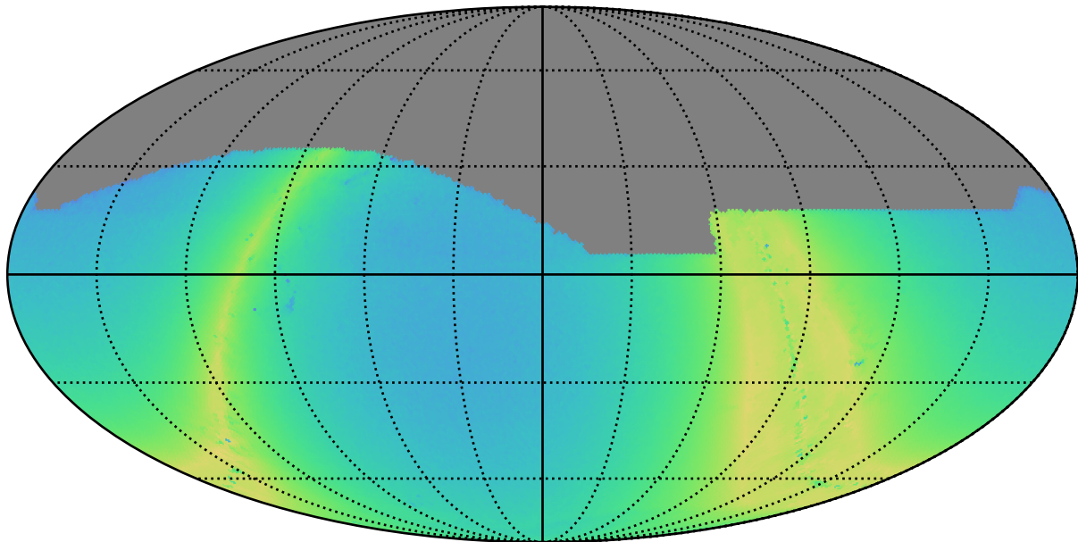
baseline_v3.2_10yrs i: N stars to Precision 0.20
