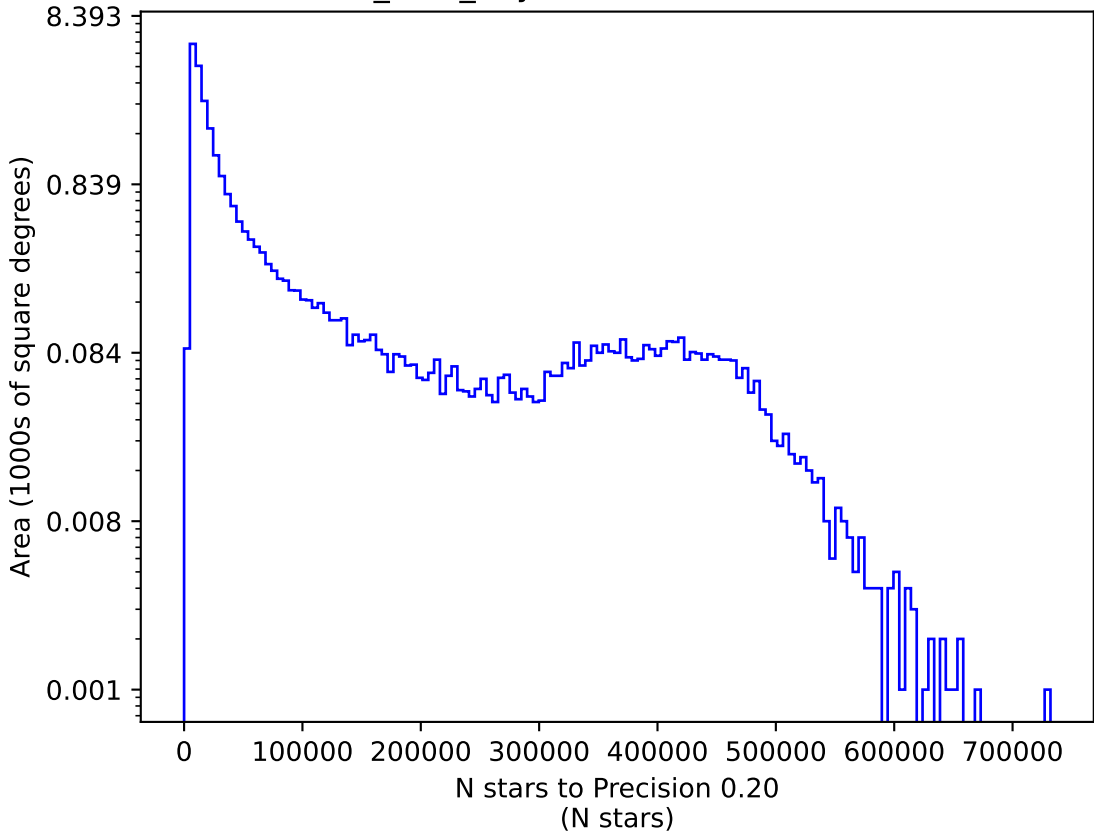
baseline_v3.2_10yrs i: N stars to Precision 0.20
