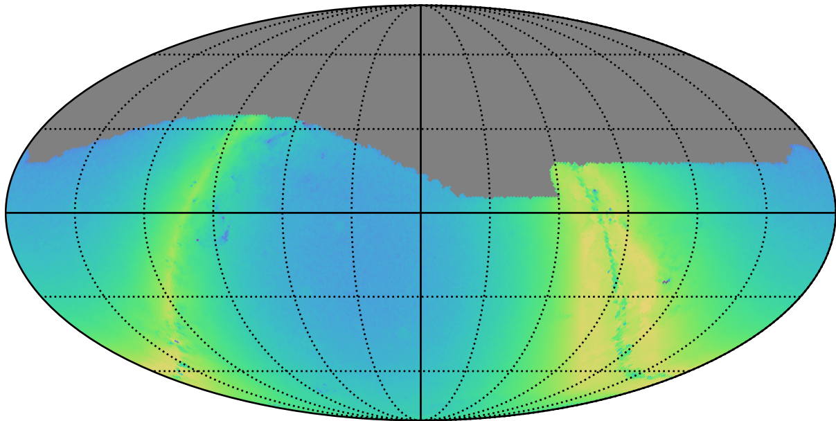
baseline_v3.2_10yrs g: N stars to Precision 0.20
