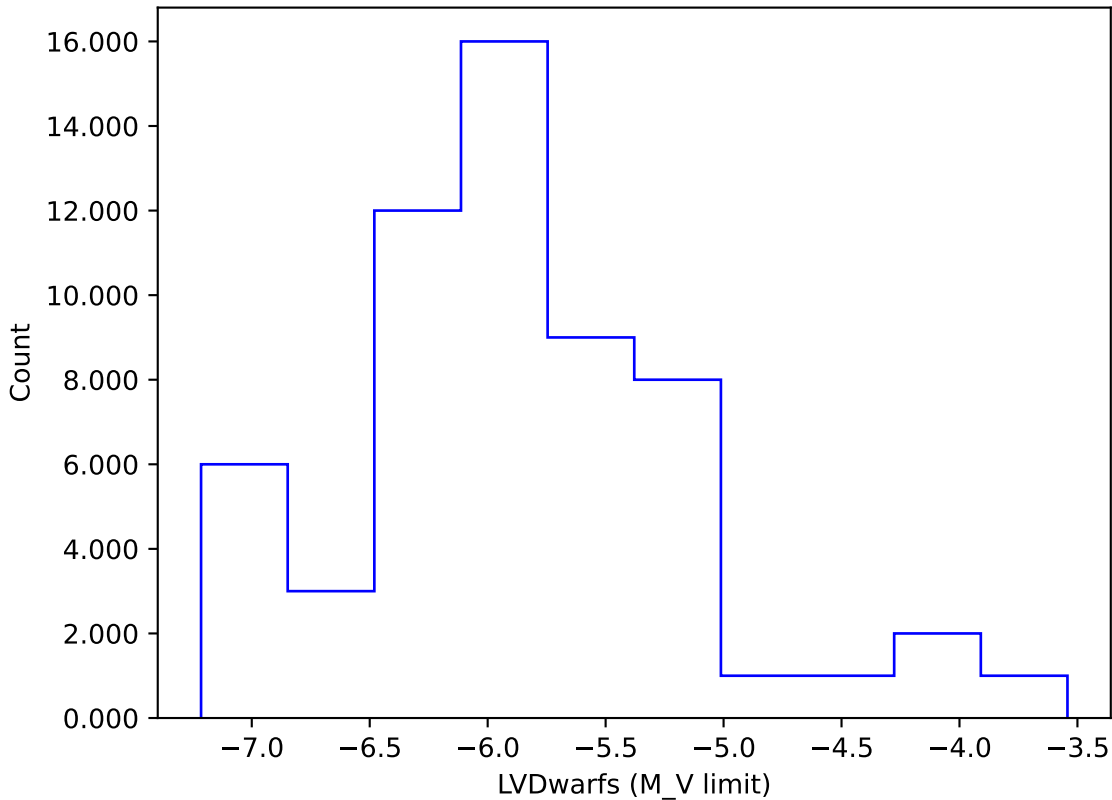
baseline_v3.2_10yrs gi: LVDwarfs
