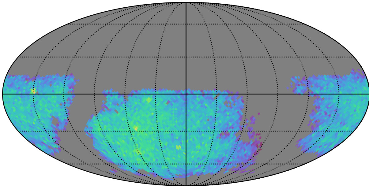
baseline_v3.2_10yrs gi: LVDwarfs
