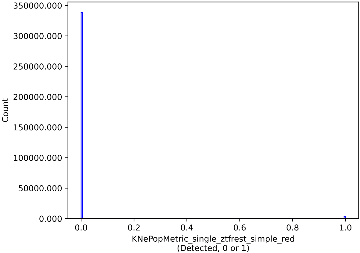
baseline_v3.2_10yrs single model: KNePopMetric_single_ztfrest_simple_red
