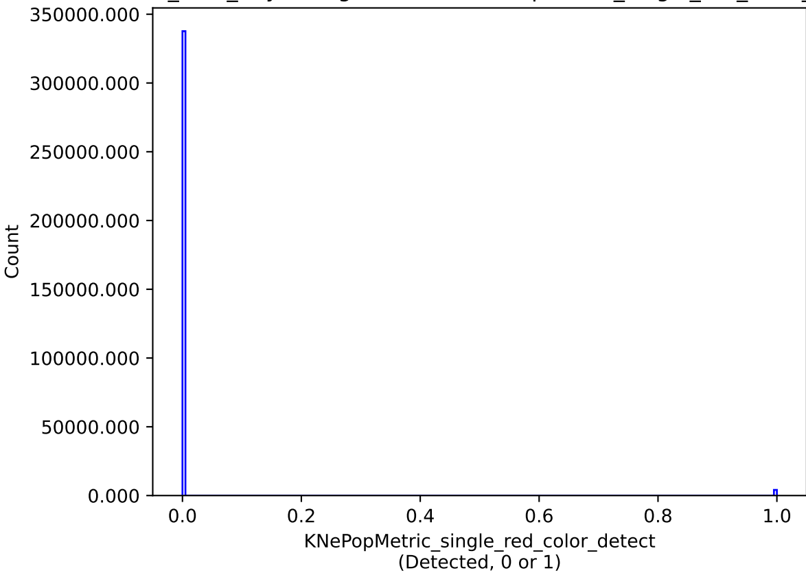
baseline_v3.2_10yrs single model: KNePopMetric_single_red_color_detect
