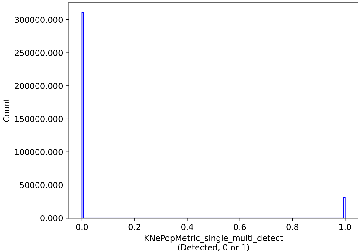
baseline_v3.2_10yrs single model: KNePopMetric_single_multi_detect
