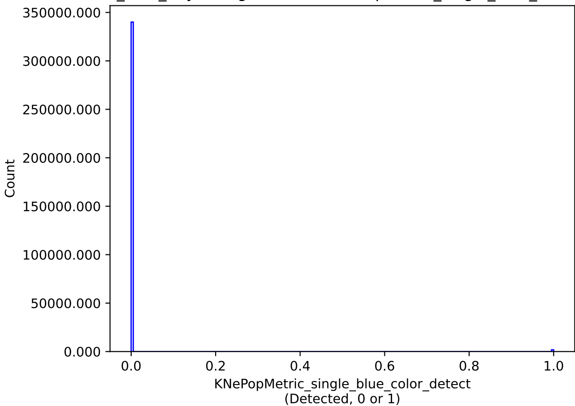
baseline_v3.2_10yrs single model: KNePopMetric_single_blue_color_detect
