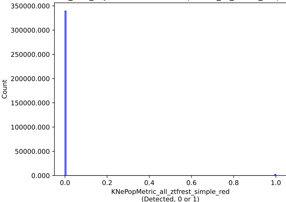
baseline_v3.2_10yrs all models: KNePopMetric_all_ztfrest_simple_red
