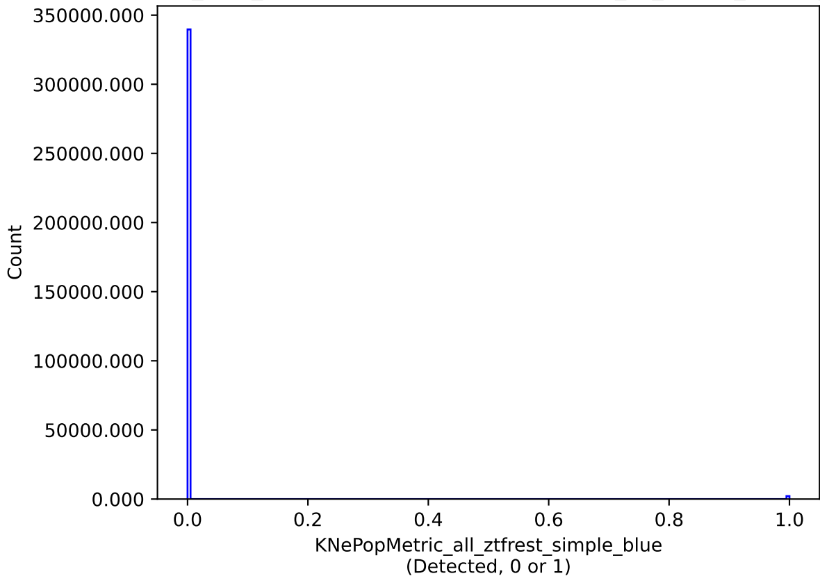
baseline_v3.2_10yrs all models: KNePopMetric_all_ztfrest_simple_blue
