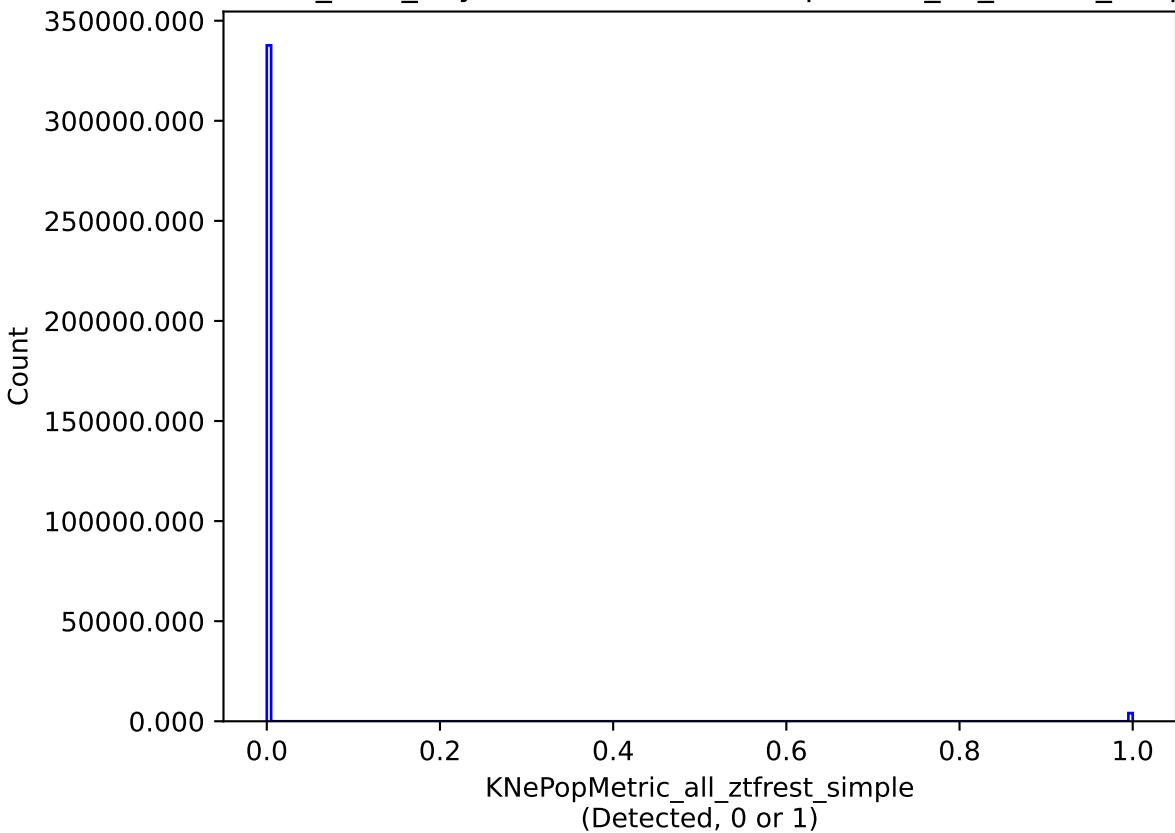
baseline_v3.2_10yrs all models: KNePopMetric_all_ztfrest_simple
