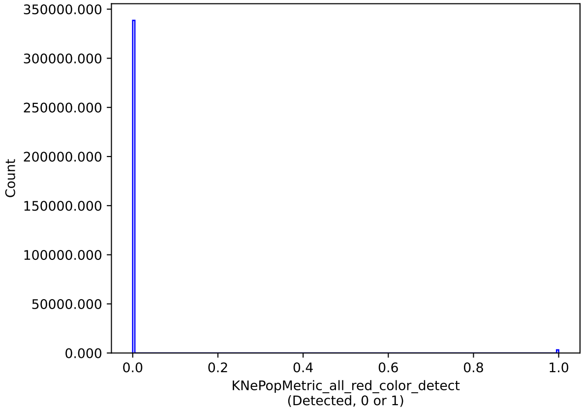
baseline_v3.2_10yrs all models: KNePopMetric_all_red_color_detect
