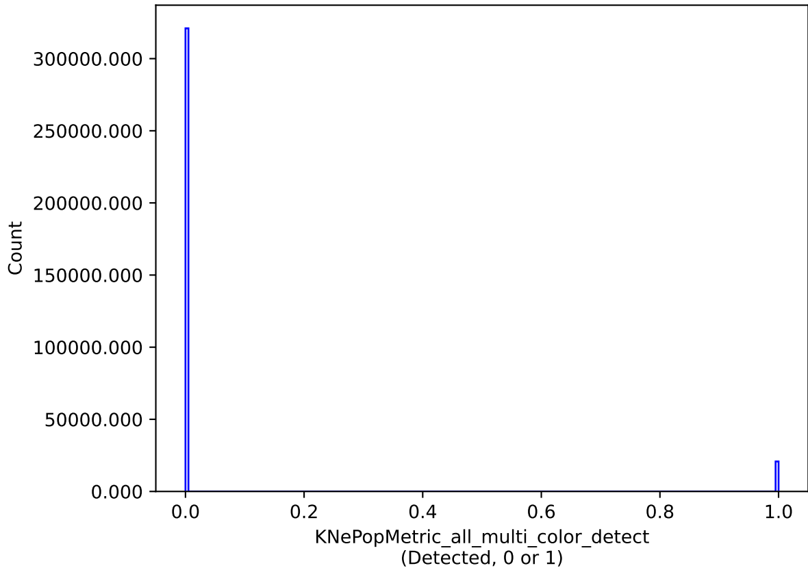
baseline_v3.2_10yrs all models: KNePopMetric_all_multi_color_detect
