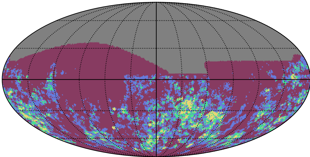
baseline_v3.2_10yrs z band: Gaps_7hr
