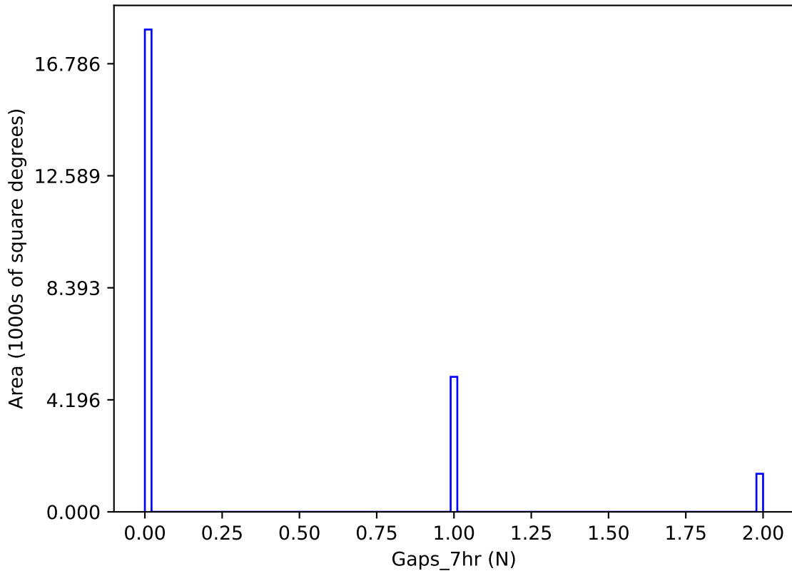
baseline_v3.2_10yrs y band: Gaps_7hr
