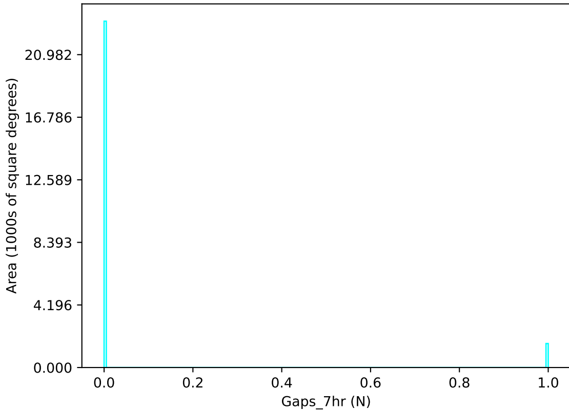
baseline_v3.2_10yrs u band: Gaps_7hr
