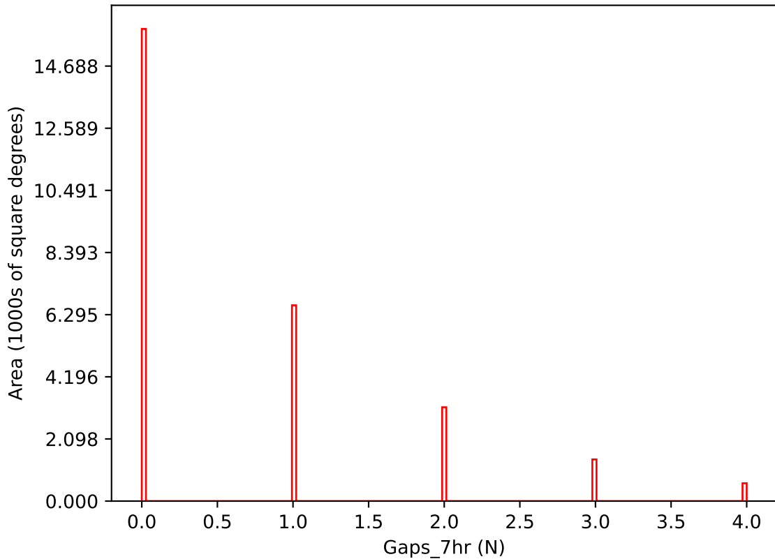
baseline_v3.2_10yrs i band: Gaps_7hr
