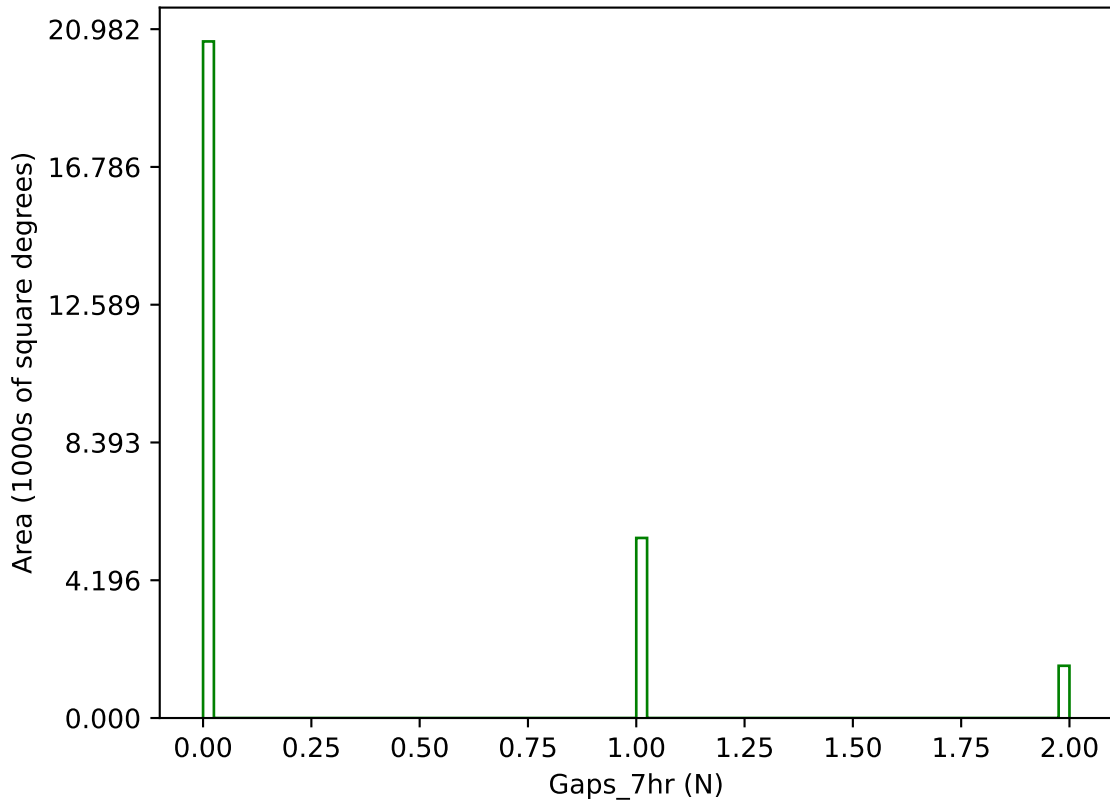
baseline_v3.2_10yrs g band: Gaps_7hr
