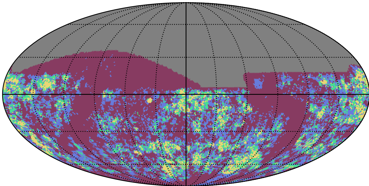
baseline_v3.2_10yrs z band: Gaps_3hr
