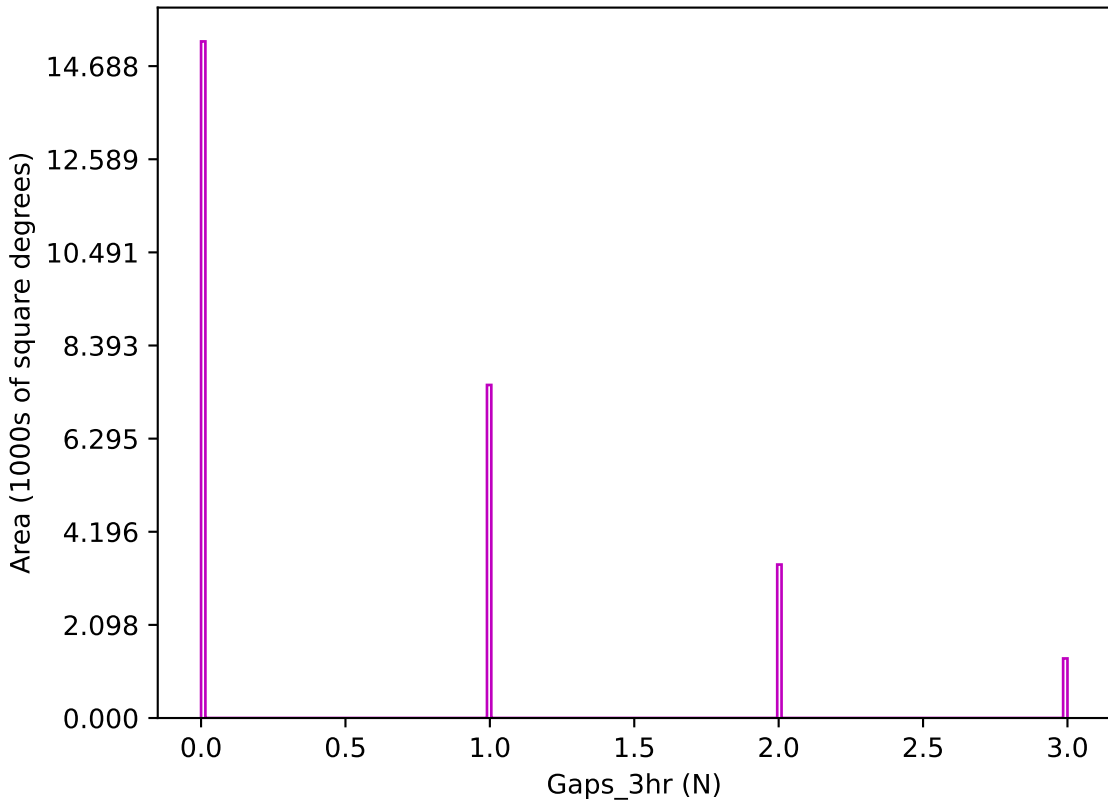
baseline_v3.2_10yrs z band: Gaps_3hr
