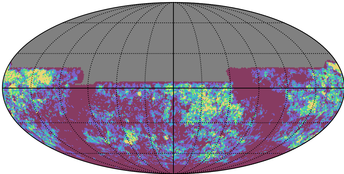
baseline_v3.2_10yrs y band: Gaps_3hr
