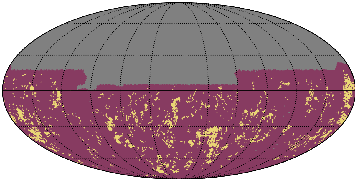
baseline_v3.2_10yrs u band: Gaps_3hr
