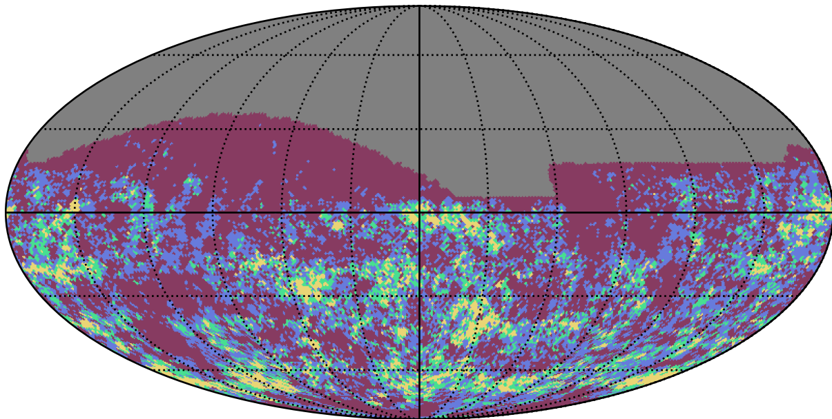
baseline_v3.2_10yrs r band: Gaps_3hr
