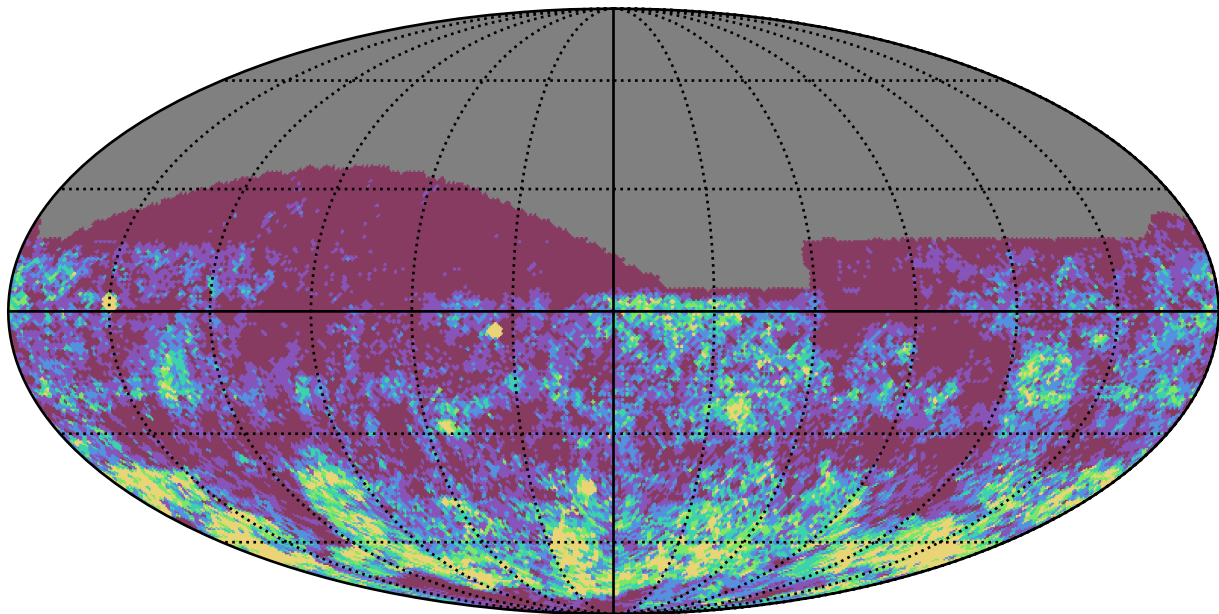
baseline_v3.2_10yrs i band: Gaps_3hr
