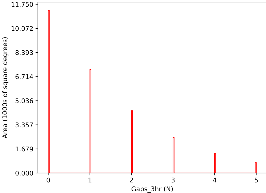
baseline_v3.2_10yrs i band: Gaps_3hr
