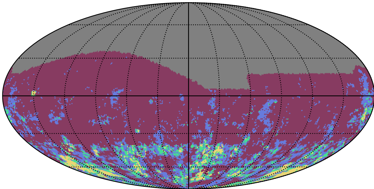
baseline_v3.2_10yrs g band: Gaps_3hr
