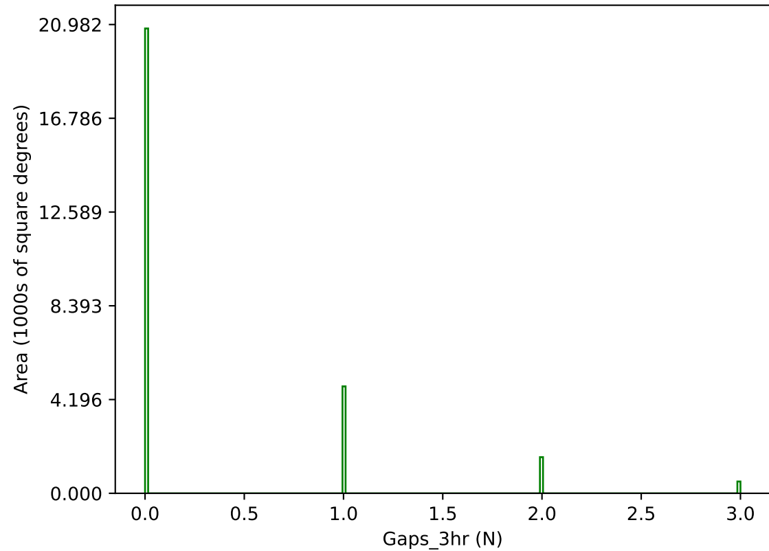
baseline_v3.2_10yrs g band: Gaps_3hr
