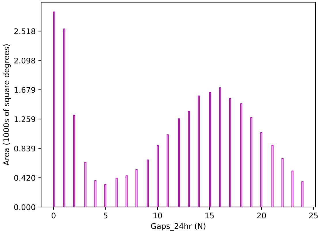
baseline_v3.2_10yrs z band: Gaps_24hr
