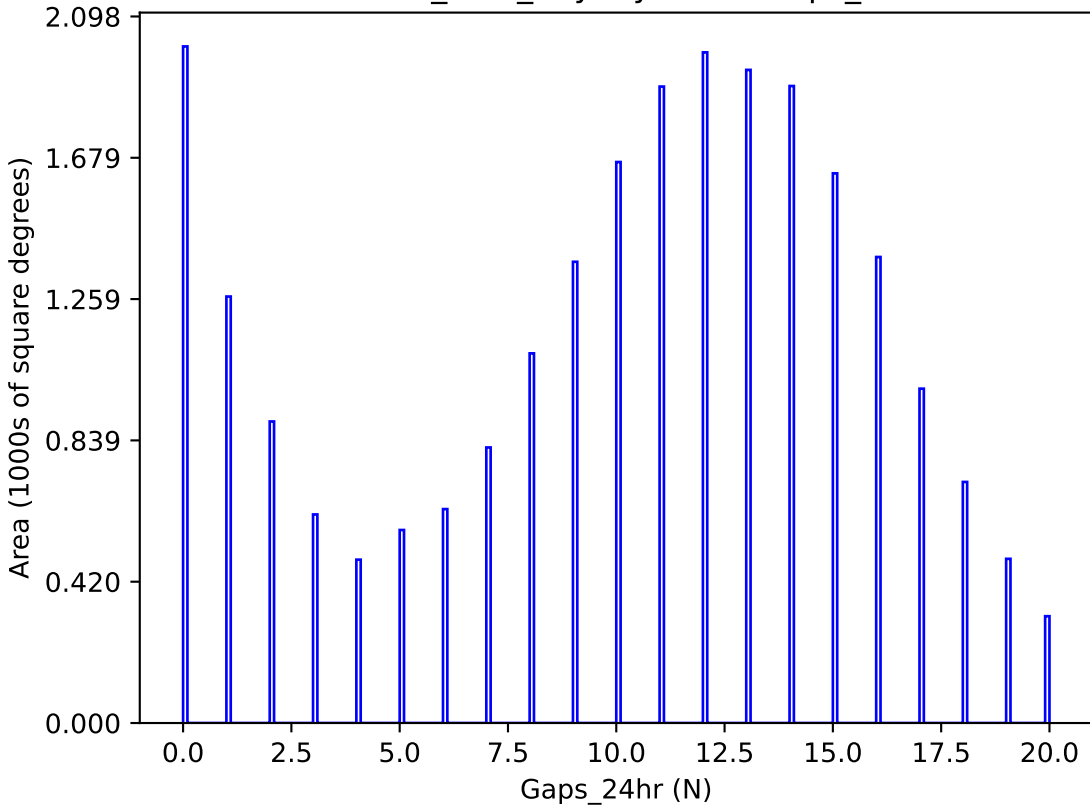
baseline_v3.2_10yrs y band: Gaps_24hr
