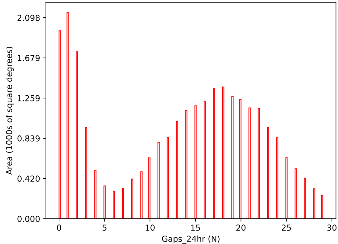
baseline_v3.2_10yrs i band: Gaps_24hr
