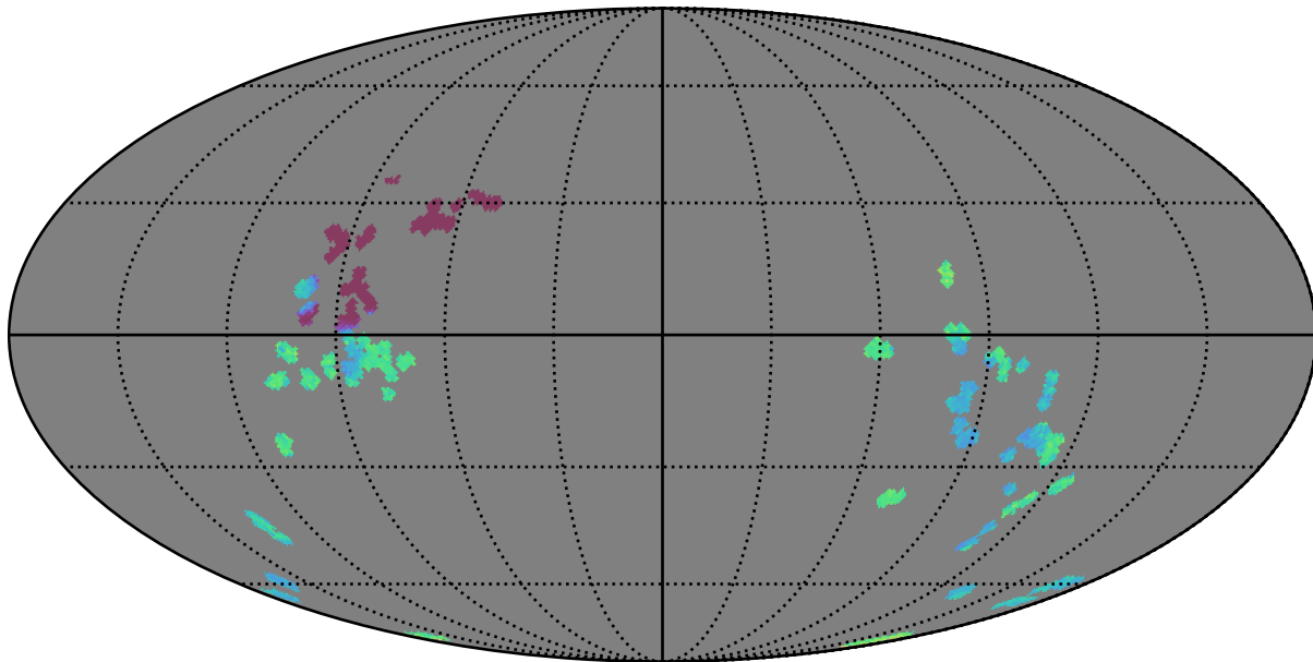
baseline_v3.2_10yrs : GalplaneTimePerFilter_zucker_sfr_map_y
