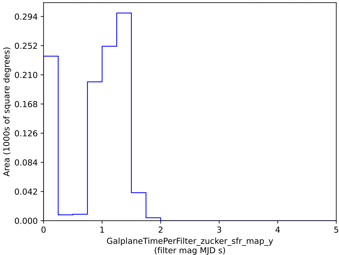
baseline_v3.2_10yrs : GalplaneTimePerFilter_zucker_sfr_map_y
