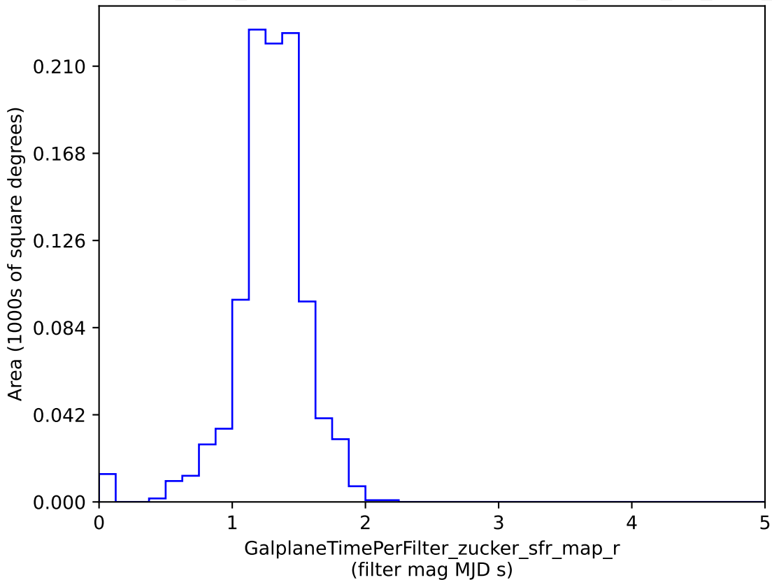
baseline_v3.2_10yrs : GalplaneTimePerFilter_zucker_sfr_map_r
